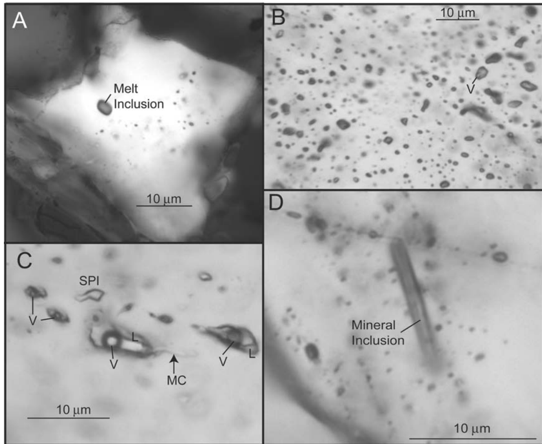
Fig. 8. Photomicrographs of inclusions in quartz. a) Melt inclusions (sample RIE030803–1.2 collected from Lehburg), single-phase aqueous inclusions (SPI in [c] sample 136 collected by Stöffler from Schratzen Hofen), b) and c) two-phase aqueous inclusions (in [b]: sample 698 collected by Stöffler from Langenmuehle), and d) mineral inclusions of rutile and apatite (sample RIE030803–1.1 collected from Lehburg) were observed in shock stage 0 rocks. Two-phase inclusions contain a liquid phase ( L ) and a vapor bubble ( V ), while melt inclusions, mineral inclusions, and single-phase inclusions do not contain a vapor bubble.
