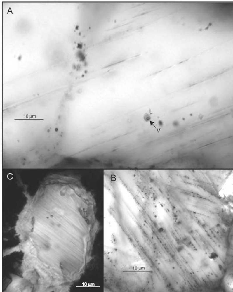
Fig. 6. Photomicrographs of shock features in quartz, illustrating the relationship of two-phase and single-phase inclusions to these features. It should be noted that most grains that contain planar fractures and/or shock lamellae do not contain inclusions and that the cases illustrated are somewhat atypical. a) Two-phase fluid inclusions are observed in a few grains which also contain planar fractures (shock stage 1, sample RIE090803-1.I from polymict breccia at Myers Keller near Noerdlingen). Single-phase inclusions are also observed in grains with (b) decorated planar fractures (shock stage 1, sample 316 collected by Stöffler from Zipplingen) and (c) shock lamellae (shock stage 3, sample RIE080803-1.II from Amuehle).
