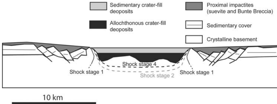
Fig. 5. Schematic cross-section of the Ries crater showing approximate shock stage isobars of interest (cross-section modified from Osinski et al. (2004), pressure estimates from Turtle and Pierazzo (1998)). Most two-phase fluid inclusions have re-equilibrated to form single-phase inclusions in shock stage 1 samples. At and above shock stage 2, most single-phase inclusions are also lost from the samples. Shock stage 4 represents whole-rock melting.
